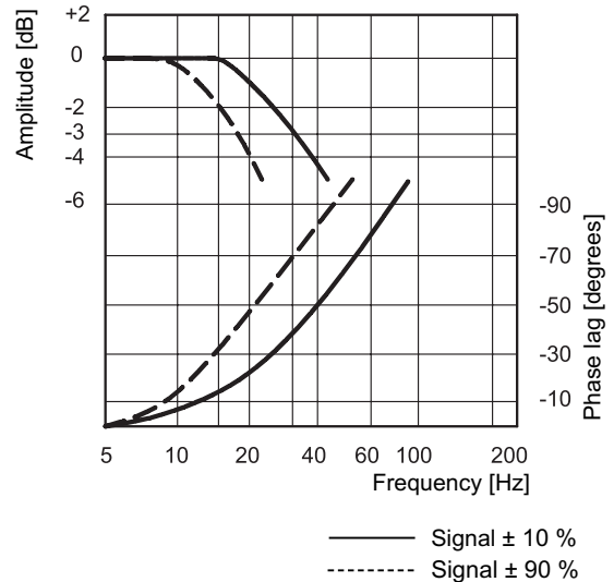
FREQUENCY RESPONSE
