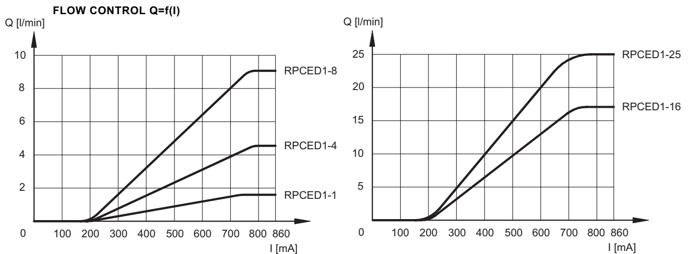
Typical curves for flow rate A → B according to the current supplied to the solenoid for controlled flow rate of: 1-4-8-16-25 l/min.
