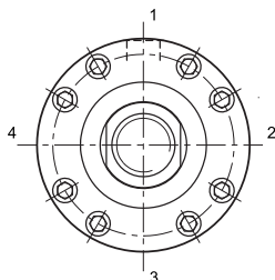
Frontal view - piston side
