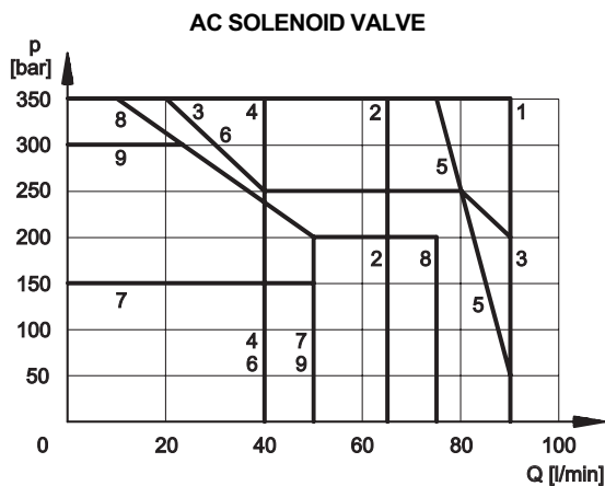
AC SOLENOID VALVE with coil A110 fed with 110V - 60 Hz
